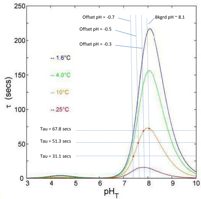
Curves from the Zeebe-Wolf Gladrow CO2 kinetic model showing e-folding time at various temperatures as a function of pH.
